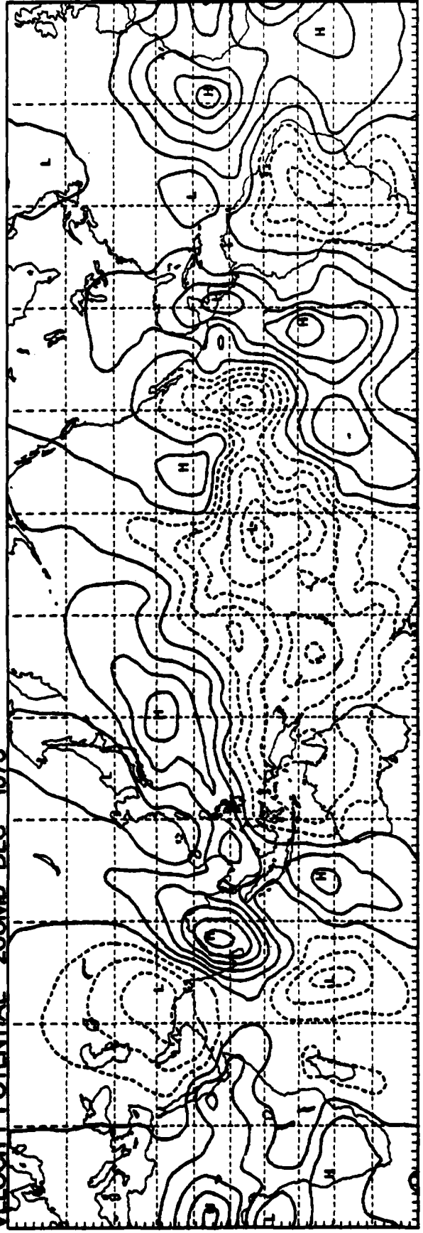
VELOCITY POTENTIAL 200MB DEC 1973
